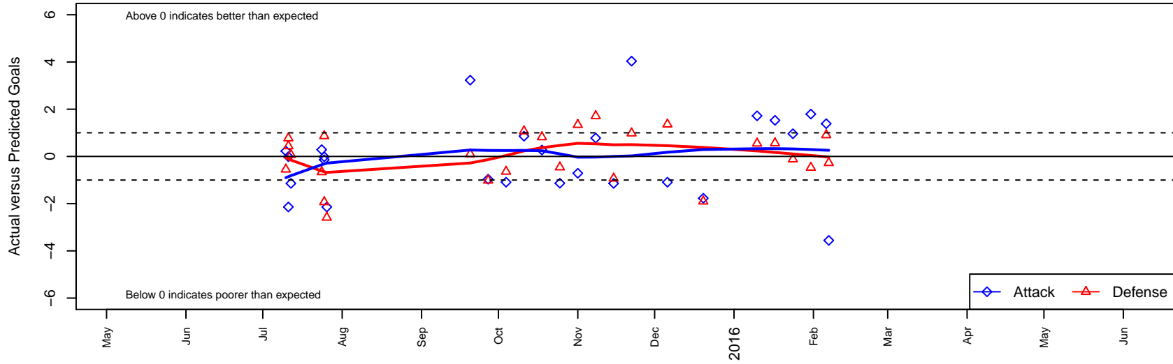
Seattle United NE Blue B00 Dots are actual minus expected GF (blue circles) and GA (red triangles). Blue line is smoothed change in attack strength. Red is smoothed change in defense strength.
